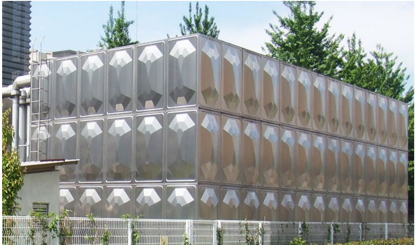
Modular water tank system made from stiffened stainless steel panels. Photo: Morimatsu (Japan), www.morimatsu.co.jp
